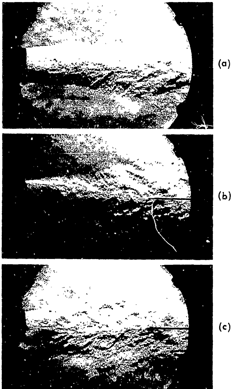
Figure 26. Schlieren photographs of the 2-inch jet seeded with \text{CO}_2 . Part (a) shows the unforced jet at an exit speed of 103 ft/sec and a Reynolds number of 106,000. The remaining parts show the jet under 2% forcing at Strouhal numbers of (b) 0.30 and (c) 0.60.
