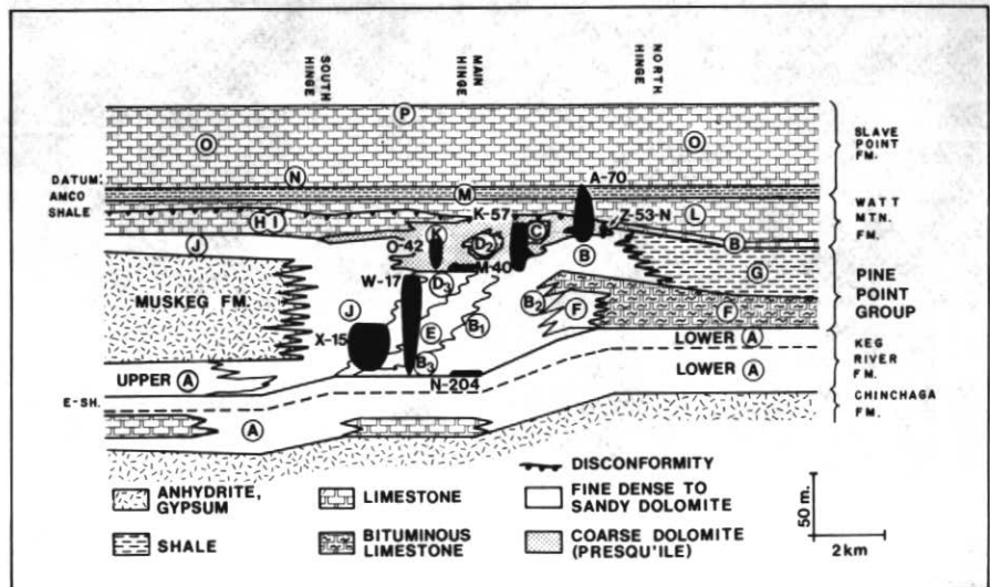
Figure 3 Schematic south-to-north cross-section through Middle Devonian Pine Point property, N.W.T., Canada, showing: division into lithologic facies A - P; main rock types; E - shale marker (Keg River Fm) and Amco Shale marker (Watt Mountain Fm) which indicate influence of hinge zones identified across top of diagram; Muskeg evaporites of Elk Point Basin to south, and G facies shales of shale basin to north; barrier complex of Facies A-L; unconformity between facies H/I and L, suggested to control karsting in underlying units; and projected stratigraphic locations of some of the major orebodies (A-70, K-57, X-15, etc.). Two facies (B, F) are rich in indigenous organic matter. Organic geochemical studies of indigenous organic matter, heavy oil and bitumen demonstrate that the carbonate barrier on the property has a low temperature history
