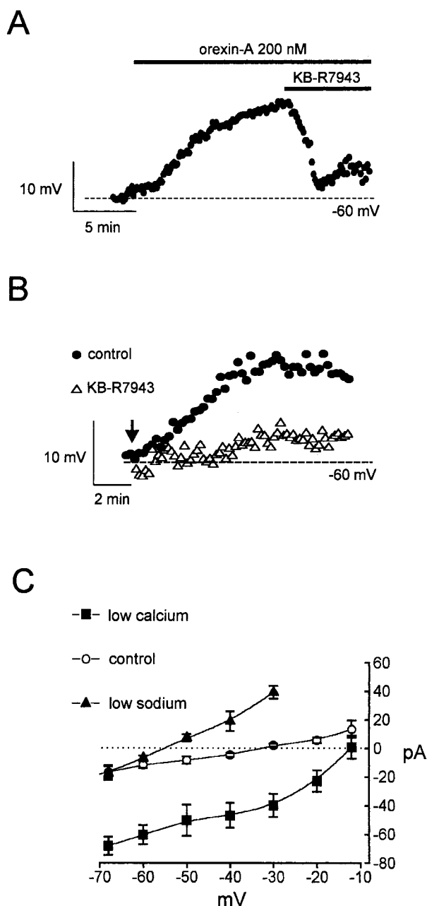
Figure 6. Orexin action is mediated by a \text{Na}^+/\text{Ca}^{2+} exchange current. Effects of the \text{Na}^+/\text{Ca}^{2+} exchange inhibitor KB-R7943 (70 \mu\text{M} ) on the depolarization induced by 200 nM orexin-A. A, B , The membrane potential was set to -60 mV before orexin application to create the same initial conditions for all neurons. A , KB-R7943 was added after orexin application. B , KB-R7943 was added 5 min before orexin application (arrowed). C , Mean current–voltage relations for the orexin-induced current in control ( n = 12 ), low external \text{Ca}^{2+} ( n = 5 ), and low external \text{Na}^+ ( n = 4 ) solutions.
