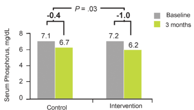
Figures 3. Schematic representation of the findings in the randomized controlled trial by Sullivan and colleagues 21 to examine the impact of nutritional education related to phosphorus additives on serum phosphorus in hyperphosphatemic patients on hemodialysis. The intervention group consisted of patients on dialysis who received education on avoidance of foods with phosphate additives or continue usual care, and the control group, patients on dialysis without this education.
