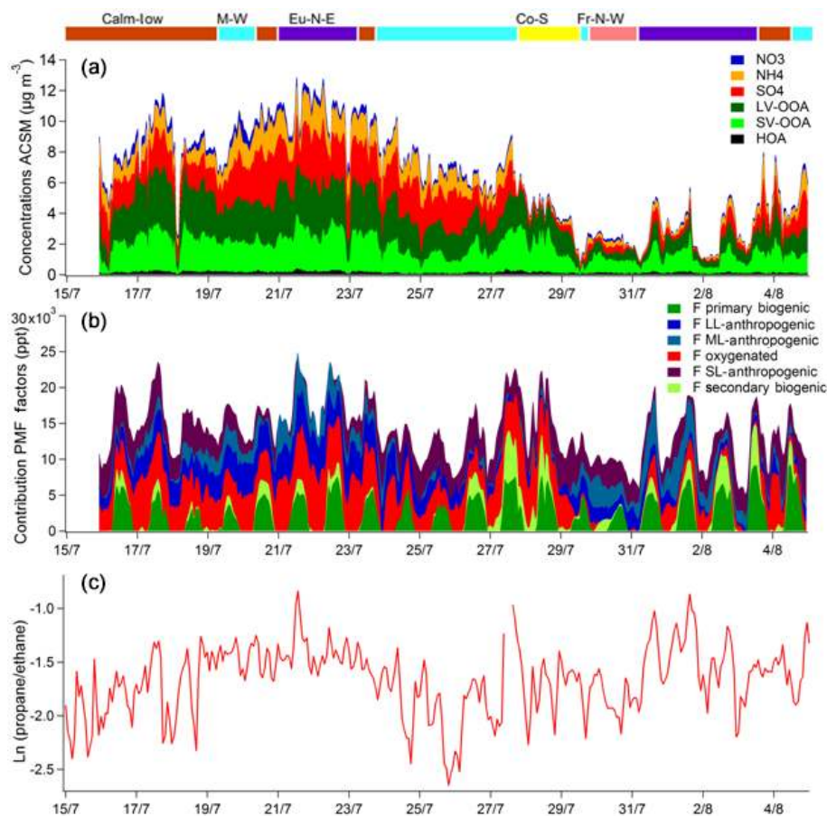
Figure 12. Stacked time series of aerosol fractions (top panel), VOC PMF factors (middle panel) and \ln(\text{propane}/\text{ethane}) as a proxy for photochemical age (bottom panel). F-LL, F-ML and F-SL anthropogenic refer to the long-lived, medium-lived and short-lived anthropogenic factors, respectively. The colored areas at the top correspond to back-trajectory clusters: light blue, purple, yellow, pink and orange-brown for the marine west (M-W), Europe northeast (Eu-N-E), Corsica south (Co-S), France northwest (Fr-N-W) and calm low wind (calm-low) clusters, respectively.
