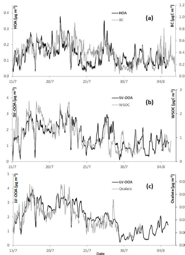
Figure 11. Time-series of (a) HOA (black) with black carbon (gray), (b) SV-OOA (black) with WSOC (gray) and (c) LV-OOA (black) with oxalate (gray).
