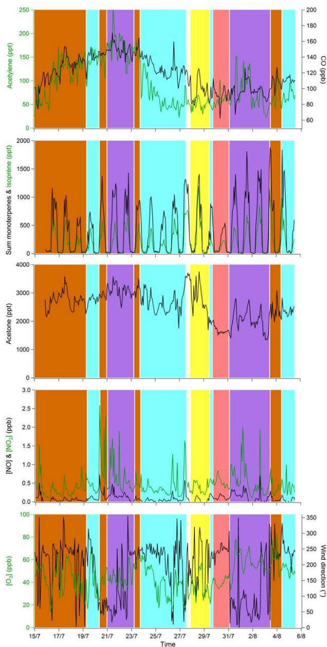
Figure 4. Time series of selected trace gases and wind direction at Cape Corse during the ChArMEs SOP2 field campaign. The colored areas correspond to back-trajectory clusters (light blue, purple, yellow, pink and orange-brown for the marine west, Europe northeast, Corsica south, France northwest and calm low wind clusters, respectively).
