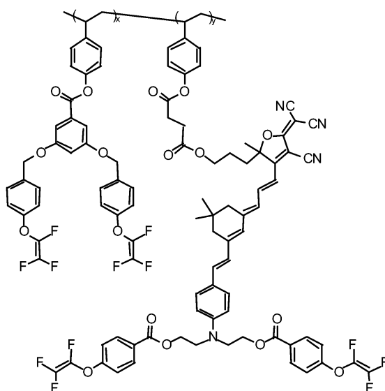
Fig. 6 The structure of a dendronized polymer leading to an electro-optic coefficient of 111 pm/V is shown. The chromophore is the CLD chromophore of ref. [21].
