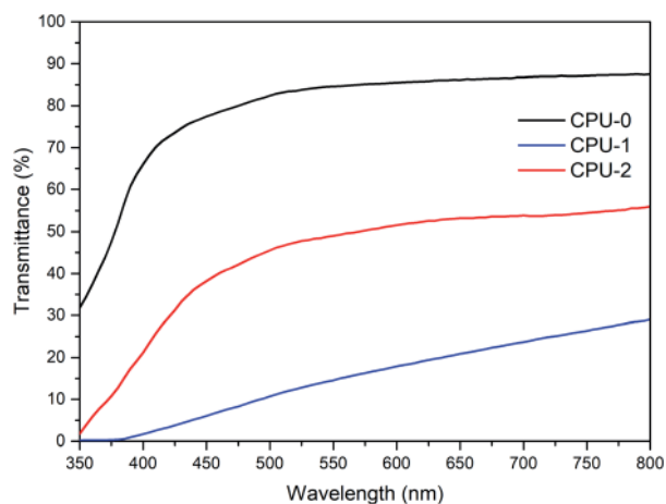
Fig. 6 Optical transmittance spectra of CPU-0, CPU-2 and CPU-1 films with thickness of 2 mm.
