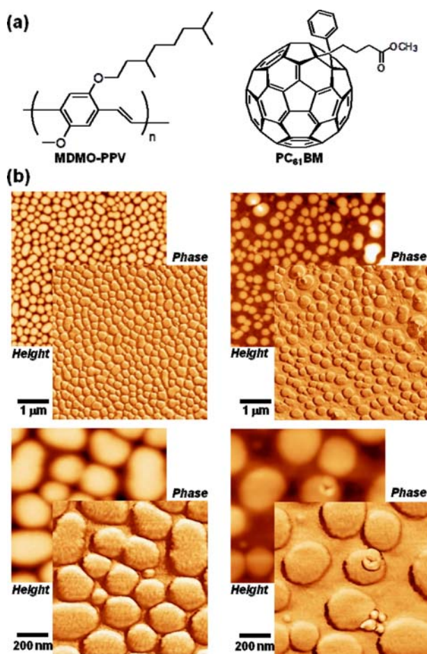
Fig. 6. (a) Chemical structure of MDMO-PPV and PC 61 BM. (b) AFM images (height and phase modes) of MDMO-PPV : PC 61 BM bulk heterojunction films prepared using chlorobenzene (left) and toluene (right): Note that individual scans were applied for each image (top: 5 μm × 5 μm, bottom: 1 μm × 1 μm).
