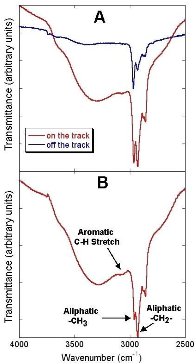
FIGURE S6 – (A) The 4000-2500 \text{cm}^{-1} spectrum from an aerogel keystone (Track 58) on a track (red line) and far from the track (blue line). The aerogel spectrum can be scaled using an absorption feature due solely to aerogel and subtracted from the track spectrum. The residual absorption (B) is then dominated by new, non-aerogel material associated with the track dominated by a broad feature near 3300 \text{cm}^{-1} (-OH) and narrower features near 3065 \text{cm}^{-1} (aromatic CH stretch, weak), 2968 \text{cm}^{-1} (-CH 3 asymmetric stretch), 2923 \text{cm}^{-1} (-CH 2 - asymmetric stretch), and 2855 \text{cm}^{-1} (symmetric -CH 3 and -CH 2 - stretches).
