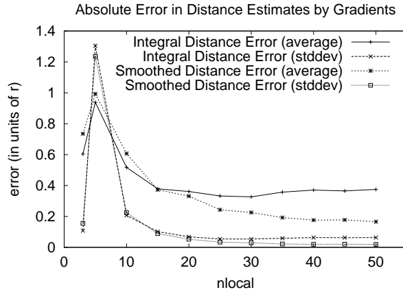
Fig. 3. Average error in gradient distance estimates for different n_{local} . Significant improvements are seen in the integral distance estimates for n_{local} < 15 . Beyond 15 there is improvement when the distance estimates are smoothed.
