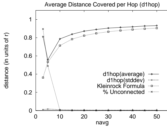
Fig. 2. Theoretical and experimental values for the average distance covered in one communication hop d_{hop} , for different expected local neighborhoods n_{local} . There is significant improvement below n_{local} = 15 , after which increasing the neighborhood size has diminishing returns.
