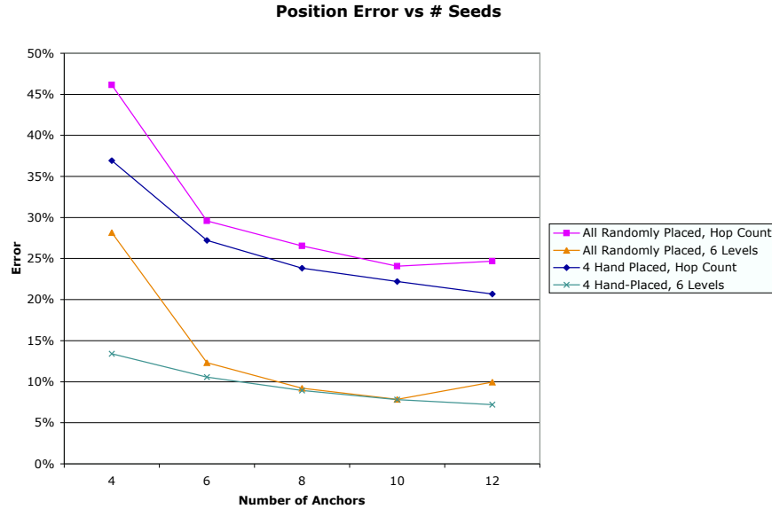
Fig. 5. Graph with position error versus number of Seeds. Position error for smoothed hop count and 6 level radio strength distance estimates are shown.
