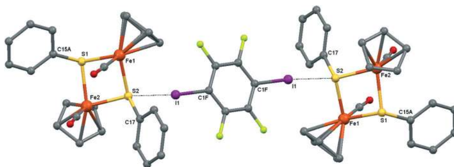
Fig. 4 Crystal structure diagram of 2, showing its I–S halogen-bonded trimolecular assemblies ([\text{CpFe}(\text{CO})(\mu_2\text{-Sph})_2(\mu_2\text{-DITFB})])_n . Hydrogen atoms are omitted for clarity. Selected distances (Å): I(1)–S(2), 3.130(1). Selected angles (°): C(1F)–I(1)–S(2), 173.9(1); Fe(1)–S(2)–I(1), 111.91(4); I(1)–S(2)–C(17), 102.5(1); I(1)–S(2)–Fe(2), 118.86(4). Dotted lines link S and I atoms at a distance shorter than the sum of the S–I vdW radii. 18
