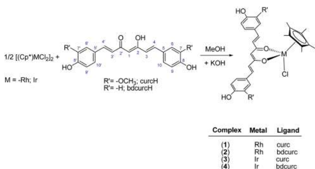
Scheme 1 Synthesis of 1–4.
