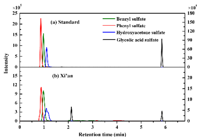
Figure 3. Typical chromatograms of organosulfates from the mixture of authentic standard solution and ambient \text{PM}_{2.5} samples, measured with the UPLC–ESI–MS/MS method. Note, the intensity of benzyl sulfate and phenyl sulfate refers to the left y axis, and the intensity of hydroxyacetone sulfate and glycolic acid sulfate refers to right y axis.
