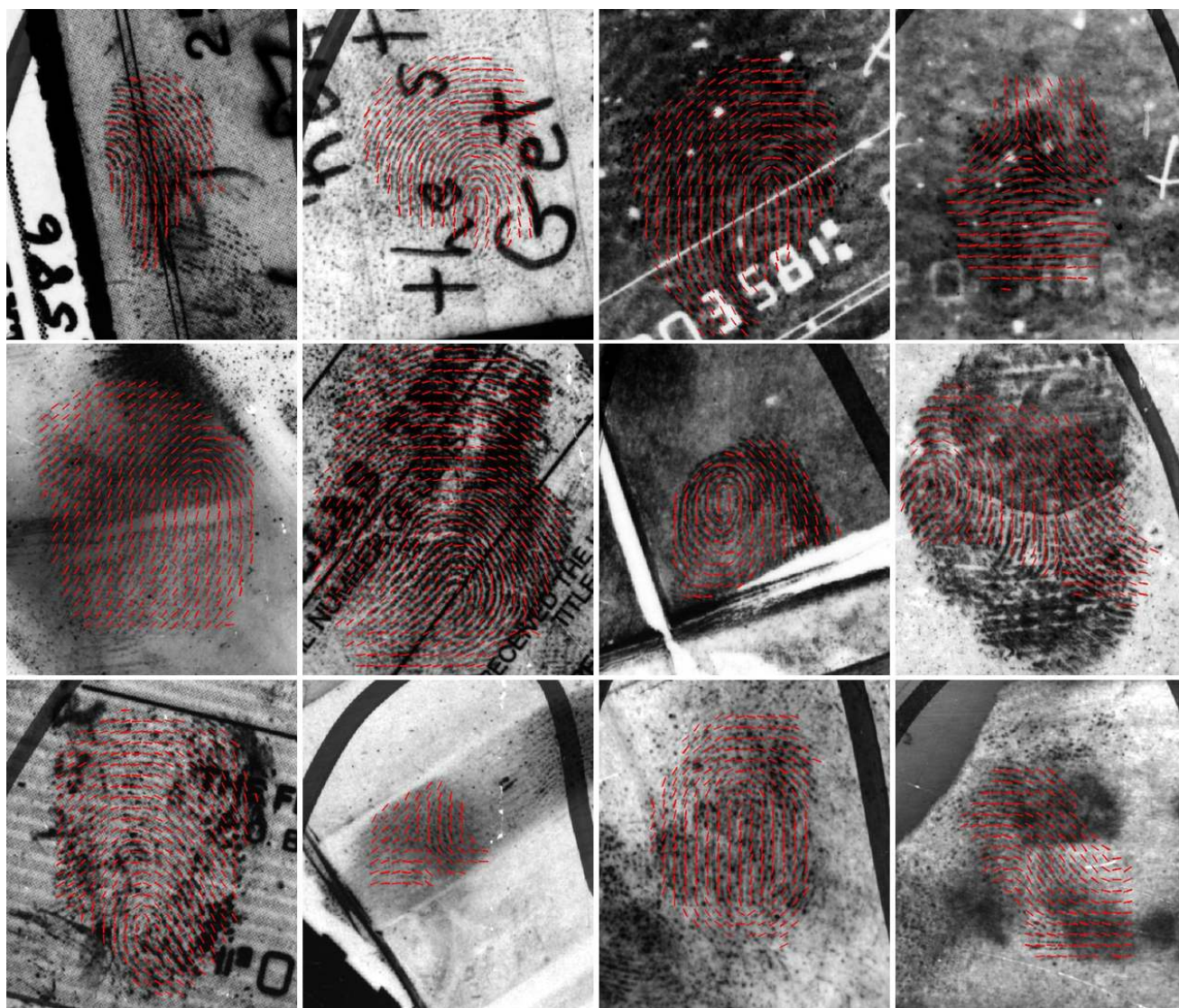
Fig. 15. Orientation fields estimated by the proposed algorithm for twelve latent fingerprints in the NIST SD27 database.
