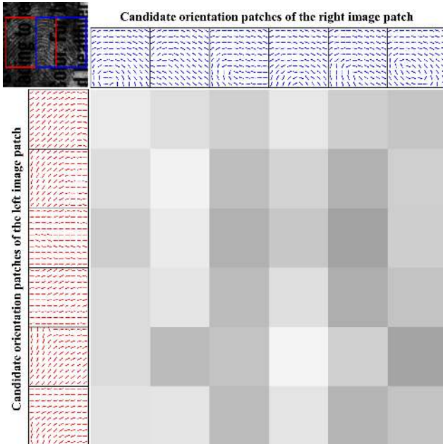
Fig. 12. Compatibility matrix between the candidate orientation patches for two neighboring patches. The compatibility value between two candidates is depicted by the brightness of the corresponding square.
