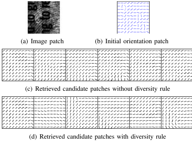
Fig. 10. Candidate orientation patches obtained without (c) and with (d) diversity rule.
