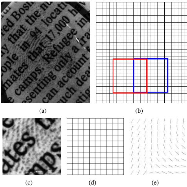
Fig. 3. A fingerprint image in (a) is divided into a number of non-overlapping blocks of 16 \times 16 pixels in (b). A patch contains 10 \times 10 blocks and neighboring patches are overlapped as shown in (b). Given a subimage in (c), the associated blocks and orientation patch is shown in (d) and (e). The orientation element represents the dominant ridge flow in a block.
