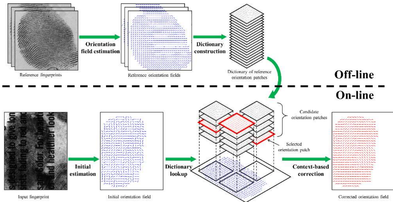
Fig. 5. The proposed system consists of an off-line dictionary construction stage and an on-line orientation field estimation stage.
