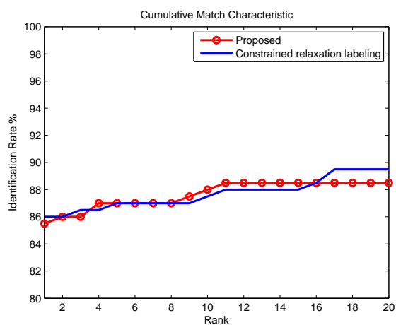
Fig. 18. CMC curves of the proposed algorithm and the constrained relaxation labeling algorithm [52] on the Tsinghua overlapped latent fingerprint database.
