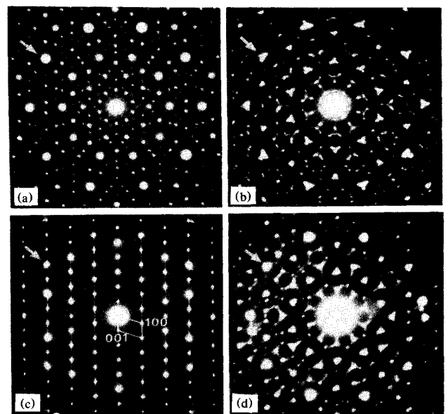
FIG. 1. Diffraction patterns from decagonal quasicrystal and \text{Al}_{13}\text{Fe}_4 twins: (a) decagonal tenfold axis, (b) tenfold twins [010], (c) single twin [010] (100 should read 200), and (d) decagonal tenfold and tenfold twins [010] axis.
