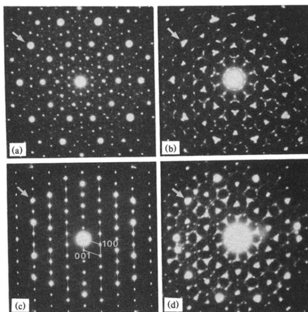
FIG. 1. Diffraction patterns from decagonal quasicrystal and \text{Al}_{13}\text{Fe}_4 twins: (a) decagonal tenfold axis, (b) tenfold twins [010] , (c) single twin [010] (100 should read 200), and (d) decagonal tenfold and tenfold twins [010] axis.
