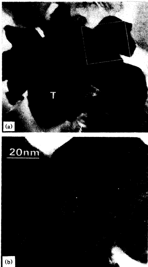
FIG. 2. (a) Intergrowth of decagonal quasicrystal ( T ) and tenfold twins of \text{Al}_{13}\text{Fe}_4 . (b) The enlarged micrograph shows fringes of five twins rotated by about 36^\circ .
