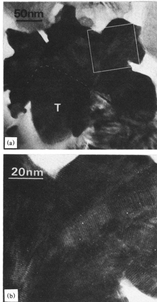
FIG. 2. (a) Intergrowth of decagonal quasicrystal ( T ) and tenfold twins of \text{Al}_{13}\text{Fe}_4 . (b) The enlarged micrograph shows fringes of five twins rotated by about 36^\circ .
