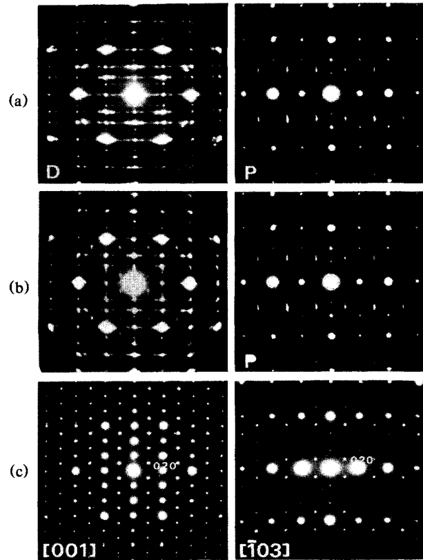
FIG. 3. Comparison of the twofold pseudo-hexagonal and pseudosquare patterns of the decagonal crystal (a), and the [001] and [\bar{1}03] patterns of the \text{Al}_{13}\text{Fe}_4 twin (c), and the composite patterns (b), showing good coincidence of spots.
