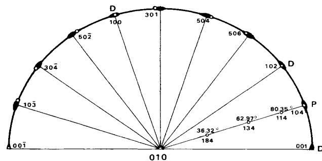
FIG. 4. Stereographic projection showing the orientation relationship between axes of the decagonal quasicrystal (solid symbols) and the \text{Al}_{13}\text{Fe}_4 twin (open circles).
