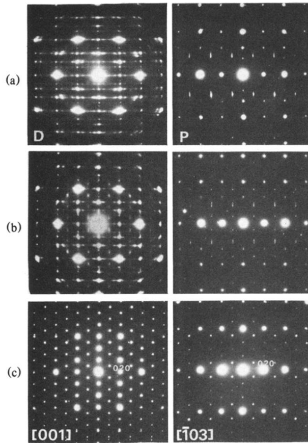
FIG. 3. Comparison of the twofold pseudo-hexagonal and pseudosquare patterns of the decagonal crystal (a), and the [001] and [\bar{1}03] patterns of the \text{Al}_{13}\text{Fe}_4 twin (c), and the composite patterns (b), showing good coincidence of spots.
