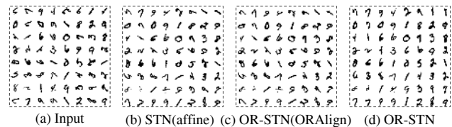
Figure 8. Orientation estimation. (a) is a mini-batch of samples from MNIST-half-rot and (b)-(d) are their rotation-rectified results.
