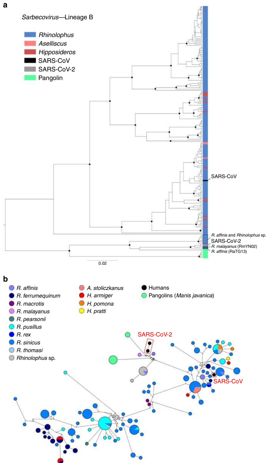
Fig. 3 Phylogenetic relationships within the Sarbecovirus subgenus ( \beta -CoVs). Maximum clade credibility tree (a) including 202 RdRp sequences from the Sarbecovirus subgenus isolated in bats, two sequences of SARS-CoV-2, and one sequence of SARS-CoV isolated in humans and eight sequences isolated in Malayan pangolins ( Manis javanica ). Well-supported nodes (posterior probability > 0.95) are indicated with a black dot. Tip colors correspond to the host genus; SARS-CoV-2 sequences and SARS-CoV sequence are highlighted in gray and black, respectively. Median-joining network (b) including 202 RdRp sequences from the Sarbecovirus lineage isolated in bats, two sequences of SARS-CoV-2, and one sequence of SARS-CoV isolated in humans and eight sequences isolated in Malayan pangolins ( Manis javanica ). Colored circles correspond to distinct CoV sequences, and circle size is proportional to the number of identical sequences in the dataset. Small black circles represent median vectors (ancestral or unsampled intermediate sequences). Branch length is proportional to the number of mutational steps between haplotypes.
