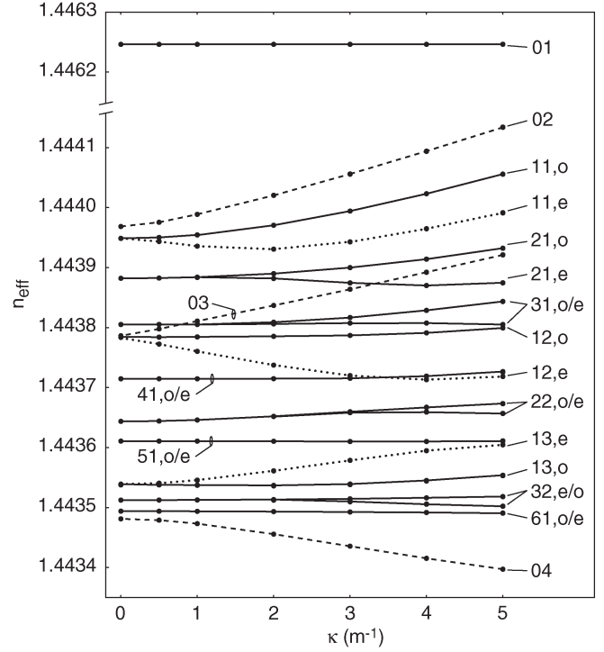
Fig. 3. Effective indexes of first 48 modes of three-layer fiber at \lambda = 1.55 \mu\text{m} . Labels indicate LP mode number and odd or even symmetry. Dashed lines indicate LP 0n cladding modes that have nonzero overlap with the core mode—and thus form attenuation notches—in a straight LPFG. Dotted lines indicate the even LP 1n cladding modes, which are responsible for the additional attenuation notches observed in bent LPFGs.
