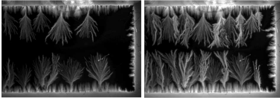
Fig. 1. MO images of flux penetration (image brightness represents flux density) into a zero-field-cooled \text{MgB}_2 film at 3.6 K. The images were taken at perpendicular applied fields of 8 (left) and 14 mT (right). See also [14].
