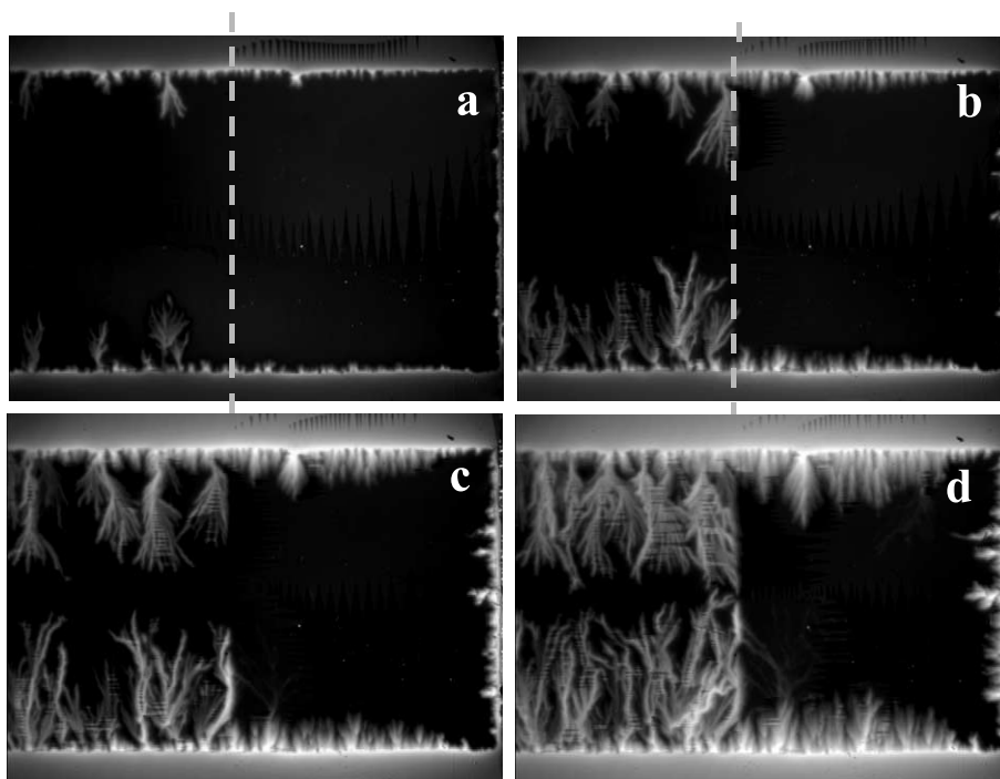
Fig. 3. (a)–(d) MO images at 3.5 K of the partly covered \text{MgB}_2 film in applied fields of 3.4, 5.0, 8.5 and 12 mT, respectively. The dashed line shows the boundary between covered and uncovered sample. Dendrite formation is suppressed where the Al-foil is in contact with the superconductor, showing the importance of thermal stabilization.
