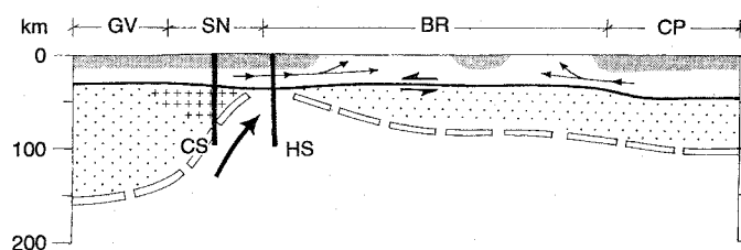
Fig. 6. Model of the late Cenozoic Cordilleran crust at latitude 36.5°N. Shading, pre-20 million-year-old upper crust; unpatterned layer with flow lines, fluid deep crust; + , eclogitic upper mantle; dots, mantle lithosphere; dashed line, 1000°C isotherm; bold arrow, locus of asthenospheric upwelling below the High Sierra; GV, Great Valley; SN, Sierra Nevada; BR, Basin and Range; CP, Colorado Plateau; CS, column of central Sierran xenolith suite; HS, column of High Sierra-Owens Valley xenolith suite.
