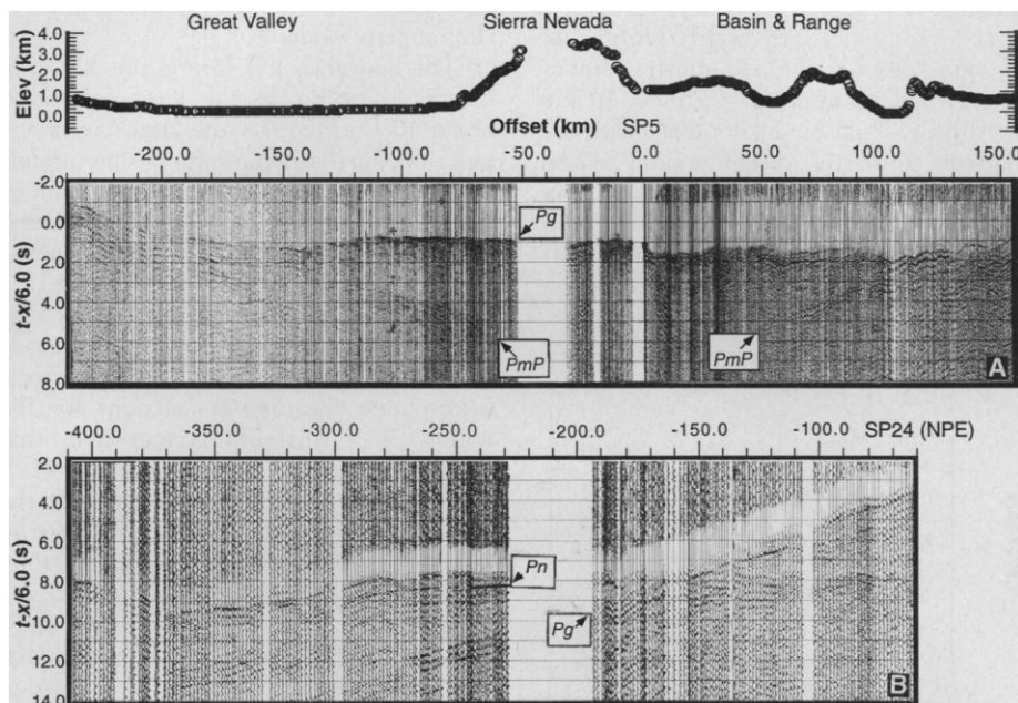
Fig. 2. East-west seismic profiles across the southern Sierra Nevada showing P_g , P_n , and P_mP phases; (A) from shot point 5 (Fig. 1); upper panel shows horizontal position and elevation of receivers; (B) from shot point 24 (nonproliferation explosion or NPE); receiver locations are approximately the same as those in (A), except east of offset -135 km receivers lie along the northwest line projecting toward the shot point (Fig. 1). Note that variations in receiver elevation and basin fill may cause small perturbations in arrival times ( <0.5 s). The delays of 1 to 2 s beneath the Great Valley in (B) are mainly due to thick Cenozoic sediments.
