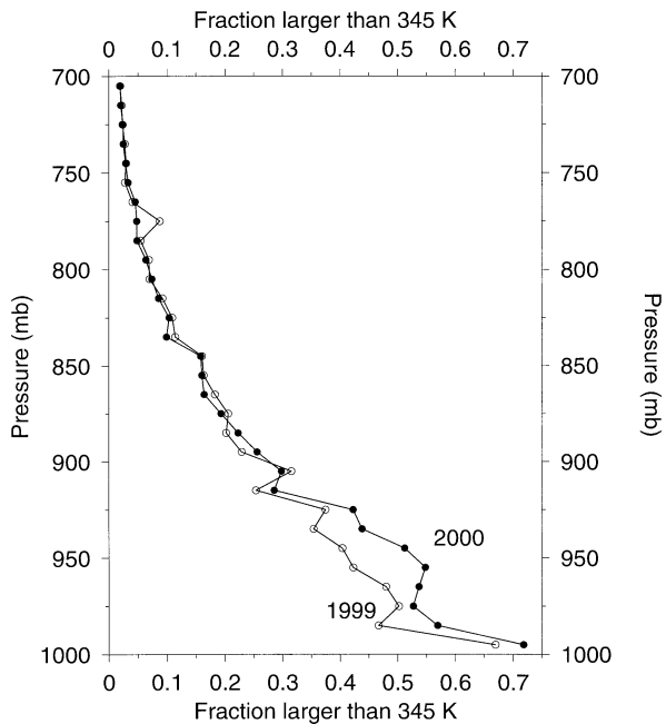
FIG. 4. The fraction of air parcels with \theta_e > 345\text{ K} , within each 10-mb interval from 1000 to 700 mb. The curve drawn in open circles was obtained from FSL NCDC data from 1999, while the curve in solid circles was obtained from 2000 data.
