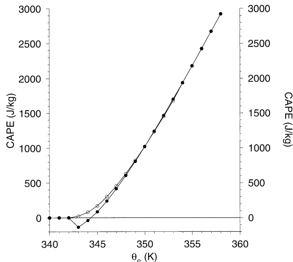
FIG. 10. The dependence of CAPE on surface \theta_e . The relative humidity of the air parcel at the surface was fixed at 0.75. The background temperature profile was an average from 15°S to 15°N. The curve with open circles refers to the CAPE as calculated from (3) in the text. The curve with solid circles was calculated by an integral from the surface rather than from the LFC, i.e., is a sum of the convective inhibition and the CAPE.
