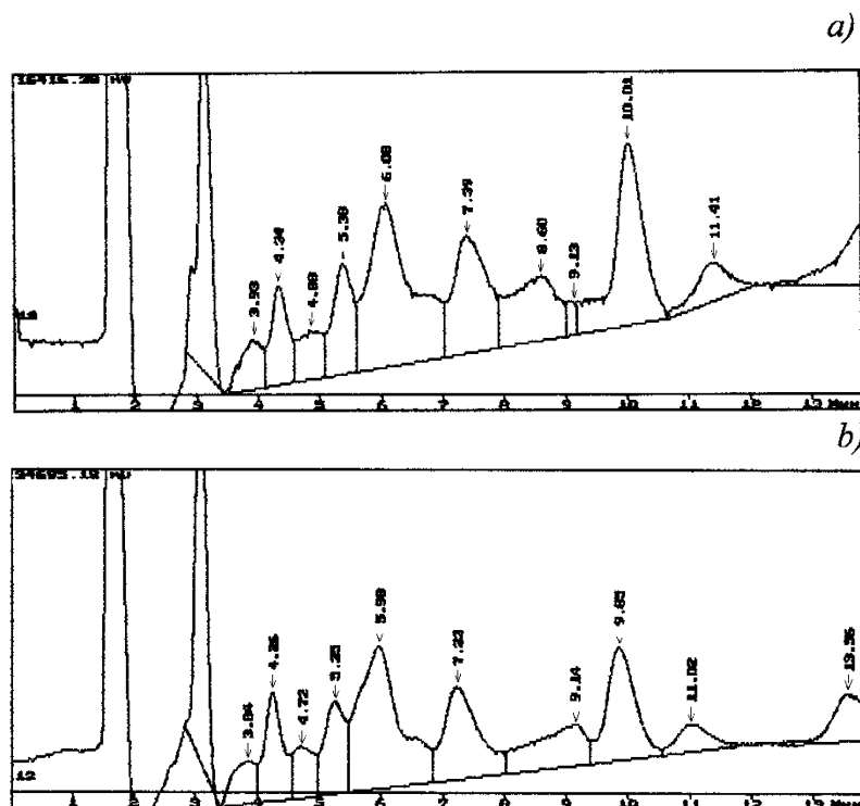
Figure 4. HPLC-chromatograms of intracellular carbohydrates obtained from protonated (a) and deuterated (b) cells of B. subtilis on the maximally deuterated D 2 O-medium: Knauer Smartline chromatograph (250×10 mm) (“Knauer”, Germany); stationary phase: Ultrasorb CN; 10 μm; mobile phase: acetonitrile–water (75:25, % (w/w); the input rate: 0.6 ml/min
