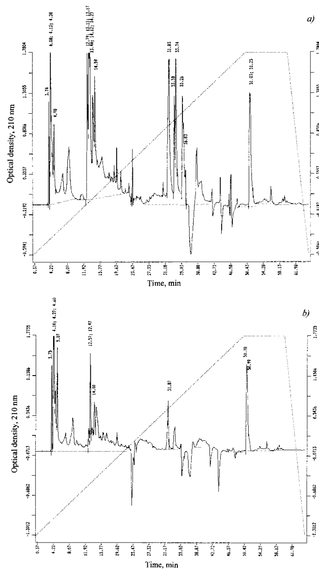
Figure 2. HPLC-chromatograms of fatty acids obtained from protonated (a) and deuterated (b) cells of B. subtilis on the maximally deuterated D 2 O-medium: Beckman Gold System (Beckman, USA) chromatograph (4.6×250 mm); stationary phase: Ultrasphere ODS, 5 μm; mobile phase: linear gradient 5 mM KH 2 PO 4 -acetonitrile (shown in phantom), elution rate: 0.5 ml/min, detection at λ = 210 nm. The peaks with retention time 3.75 min (instead of 3.74 minutes in the control), 4.10; 4.27; 4.60 (instead of 4.08; 4.12; 4.28 in the control), 5.07 (instead of 4.98 in control) 12.57; 12.97 (instead of 12.79; 13.11; 13.17 in control) 14.00 (instead of 14.59 in the control), 31.87 (instead of 31.83 in the control); 33.38; 33.74; 33.26; 36.03; 50.78; 50.99 (instead of 51.03; 51.25 for control) correspond to individual intracellular fatty acids
