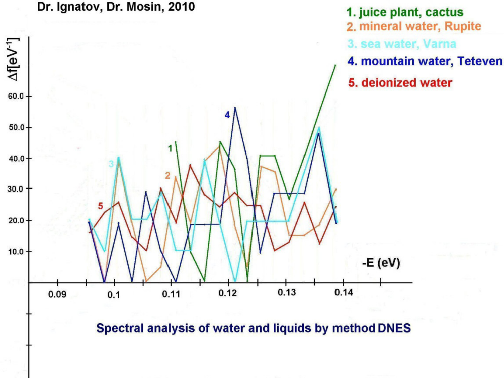
Figure 6. DNES-spectra of water samples of various origin: 1 – cactus juice; 2 – mineral water from Rupite village (Bulgaria); 3 – seawater (Varna, Bulgaria); 4 – mountain water (Teteven, Bulgaria); 5 – deionized water (the control)
