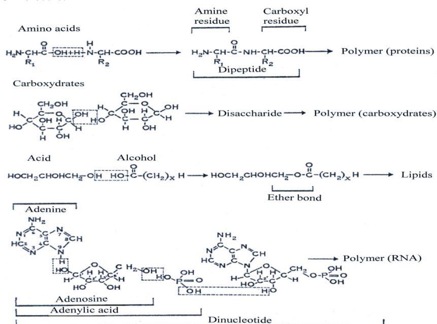
Figure 10. Reactions of condensation and dehydration in alkaline conditions with pH = 9–10 catalyzed by HCN and its derivatives, resulting in synthesis from separate molecules larger organic molecules of polymers. The top three equations: condensation and the subsequent polymerization of amino acids in proteins; carbohydrates – in polycarboxydrates and acids and ethers – into lipids. The bottom equation – condensation of adenine with ribose and H 3 PO 4 , leading to formation of dinucleotide
