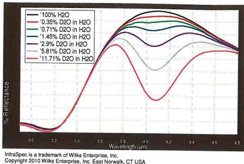
Figure 9. The typical IR-spectra of water with varying content of deuterium
