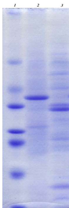
Figure 5. Electropherograms of proteins isolated from hydrolysates of total biomass of B. subtilis : 1 – a standard set of proteins; 2 – a sample obtained from protonated medium; 3 – a sample obtained from D 2 O-medium
