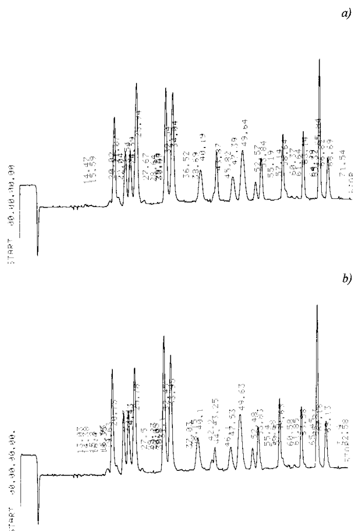
Figure 3. HPLC-chromatograms of amino acids obtained from hydrolyzates of protonated (a) and deuterated (b) cells of B. subtilis on the maximally deuterated D 2 O-medium: Biotronic LC-5001 (230×3.2 mm) column (“Eppendorf–Nethleler–Hinz”, Germany); stationary phase: UR-30 sulfonated styrene resin (“Beckman–Spinco”, USA); 25 μm; 50–60 atm; mobile phase: 0.2 N sodium–citrate buffer (pH = 2.5); the eluent input rate: 18.5 ml/h; the ninhydrin input rate: 9.25 ml/h; detection at λ = 570 and λ = 440 nm (for proline).
