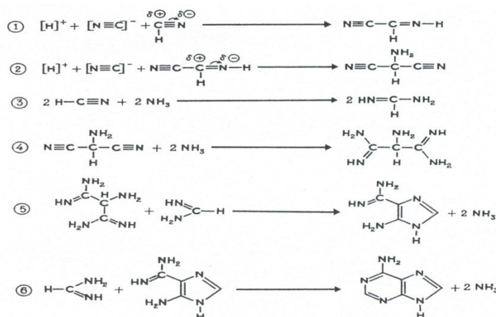
Figure 11. Prospective mechanisms of thermal (+95 °C) synthesis of purines in aqueous solutions: a) – synthesis of hypoxanthine, adenine, guanine and xanthine from 4-aminoimidazole-5-carboxamide, 4-aminoimidazole-5-carboxamide, water, NH 3 , formamidine and urea; b) – synthesis of adenine from NH 3 and HCN (total reaction: 5HCN = adenine)
