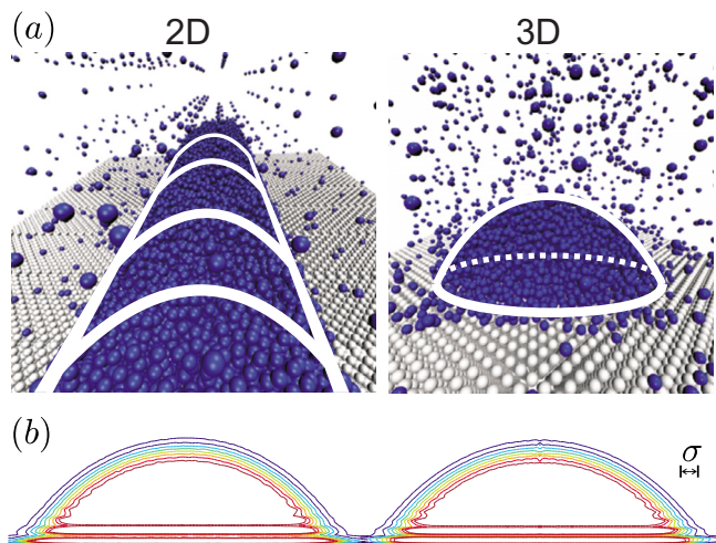
FIG. 3. (Color online) (a) Snapshots from molecular dynamics simulations of a 2D, cylindrical cap-shaped droplet (left), and a 3D, spherical cap-shaped droplet (right). The light spheres represent the immobilized solid particles, forming the substrate to which the droplet attaches. The darker spheres represent the mobile fluid particles. The lines are a guide to the eye. Several periods of the 2D droplet are shown (periodic boundary conditions), causing the same particle to be printed multiple times. These drops were simulated using identical interaction parameters ( \epsilon_{SL}/\epsilon_{LL} = \frac{2}{3} \Rightarrow \theta_Y \approx 65^\circ ) and differ in shape only because of the difference in the periodic boundary conditions. (b) Isodensity contours measured using statistical averaging from the droplets shown in the top row. The contact angle and the overall shape of the two drops are almost identical, requiring a precise measurement to observe the effect of line tension.
