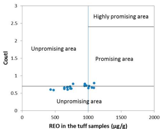
Figure 13. Evaluation of REY in the studied samples in the Lvshuidong mine. C_{outl} = [(\text{Nd} + \text{Eu} + \text{Tb} + \text{Dy} + \text{Er} + \text{Y})/\Sigma\text{REY}]/[(\text{Ce} + \text{Ho} + \text{Tm} + \text{Yb} + \text{Lu})/\Sigma\text{REY}] .
