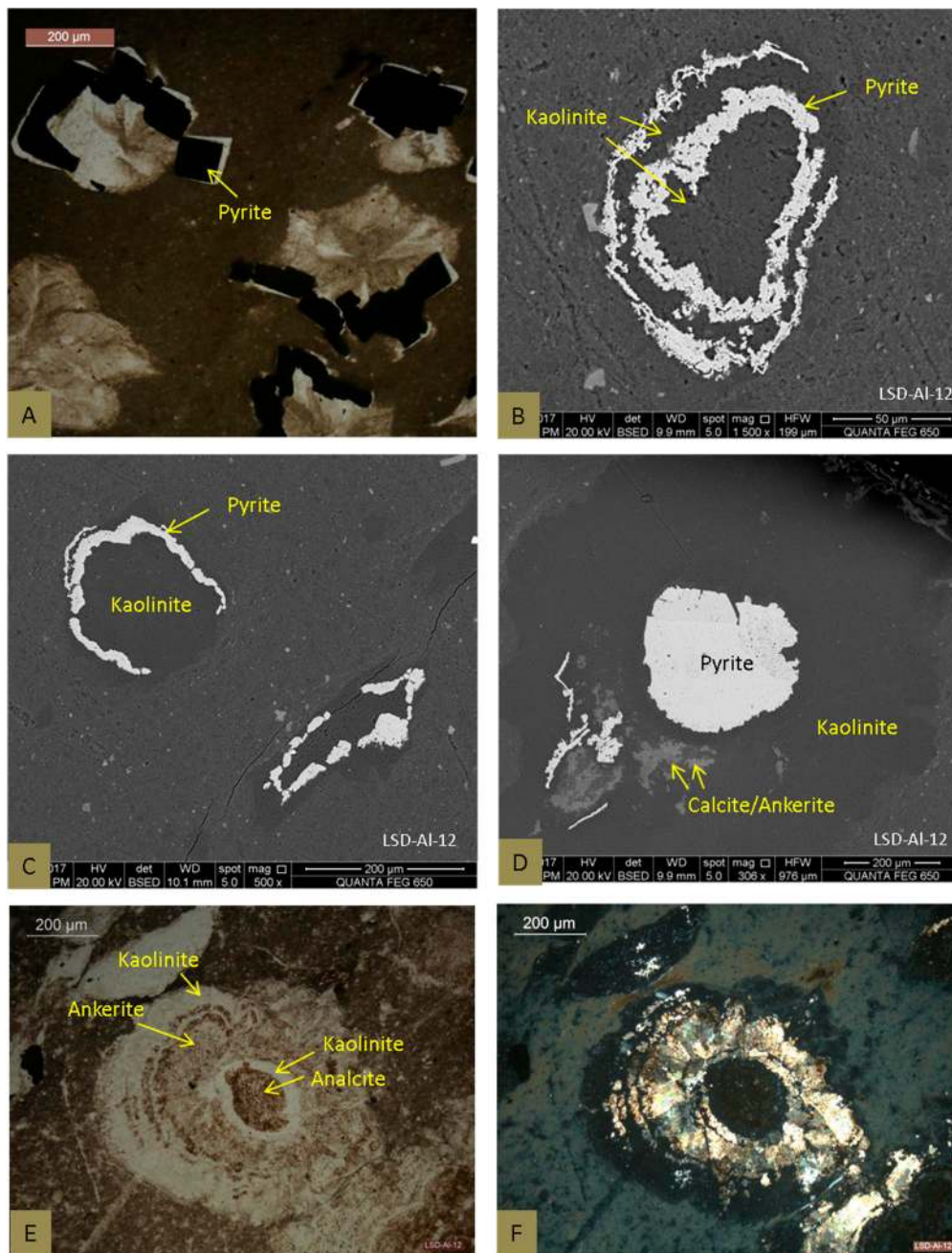
Figure 8. Images of minerals in the sample 12. (A) PPL image of pyrite overprint clay concretions; (B) SEM backscattering image of pyrite surrounded by kaolinite and carbonate minerals; (C,D) SEM backscattering images of kaolinite with pyrite rim(s); (E) PPL image of concretion consisting of analcite, kaolinite and ankerite; (F) XPL image of (E).
