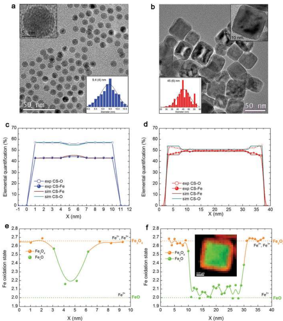
Fig. 1 TEM images of the CS nanoparticles: (a) CS 9 and (b) CS 45 . Shown in the insets are the histograms of the corresponding particles (bottom) and HRTEM images of a single particle (top). The number of particles used to obtain the particle size distribution is about 150. Elemental quantification along the particle diameter for Fe (filled circles) and O (empty circles) of (c) CS 9 and (d) CS 45 particles. The solid lines represent the simulated elemental profile for a particle with a Fe x O-3 nm/Fe 3 O 4 -3.5 nm and a Fe x O-20 nm/Fe 3 O 4 -8 nm core/shell structure for CS 9 and CS 45 particles, respectively. Fe oxidation state along the particle diameter of (e) CS 9 and (f) CS 45 particles. Shown in the inset of (f), is an EELS-mapping of CS 45 nanoparticles (where green corresponds to the O K signal corresponding to Fe x O and orange to the O K signal of Fe 3 O 4 after background subtraction using a power law fit).
