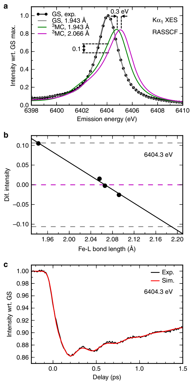
Fig. 6 Simulated \text{K}\alpha XES signals. a Experimental XES spectra of the [\text{Fe}(\text{bimp})_2]^{2+} ground state (GS, black dots), compared with the calculated GS spectrum (gray line) and the ^3\text{MC} excited state spectra at the GS geometry (green line) and at the ^3\text{MC} geometry (magenta line). b Calculated ^3\text{MC} state XES intensity change at 6404.3 eV as a function of the Fe-ligand (L) bond length, relative to the optimal ^3\text{MC} structure (black dots; black line: linear fit). Dashed lines correspond to the intensity changes at optimal (magenta) and extremal (gray) bond lengths, R = 2.066 \pm 0.123 \text{ \AA} . c Simulation of \text{K}\alpha XES time-dependent intensity at 6404.3 eV (black line: experiment; red line: simulation).
