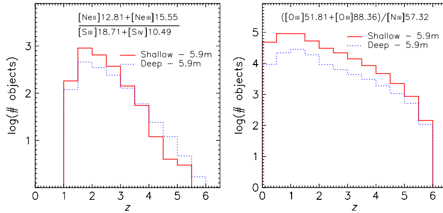
Figure 16. Left panel: predicted redshift distributions of galaxies detected simultaneously in the [Ne III] 12.81, [Ne III] 15.55, [S III] 18.71, and [S IV] 10.49 \mu\text{m} lines by the shallow (10 \text{deg}^2 ) and deep (1 \text{deg}^2 ) surveys with a 5.9 m telescope. Both surveys have a total amount of observing time equal to 1000 h. Right panel: the same, but for the simultaneous detection of the [O III] 51.81, [O III] 88.36, and [N III] 57.32 \mu\text{m} lines.
