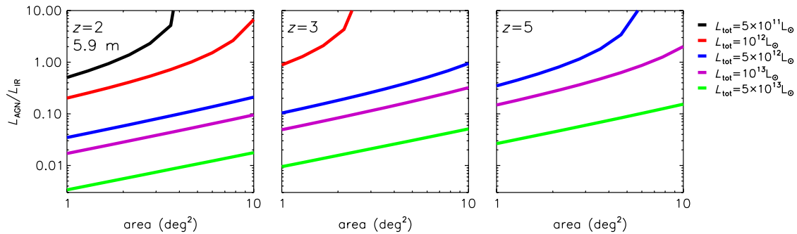
Figure 17. Minimum ratios of AGN bolometric luminosities to SF IR luminosity L_{\text{IR}} \equiv L_{\text{IR,SF}} for which lines associated with both components (the [O IV] 25.89 \mu\text{m} and the [O III] 88.36 \mu\text{m} lines, respectively) are detectable with the OST/OSS at z=2 (left), z=3 (centre), and z=5 (right), as a function of the mapped area for five values of L_{\text{tot}} = L_{\text{AGN}} + L_{\text{IR,SF}} .
