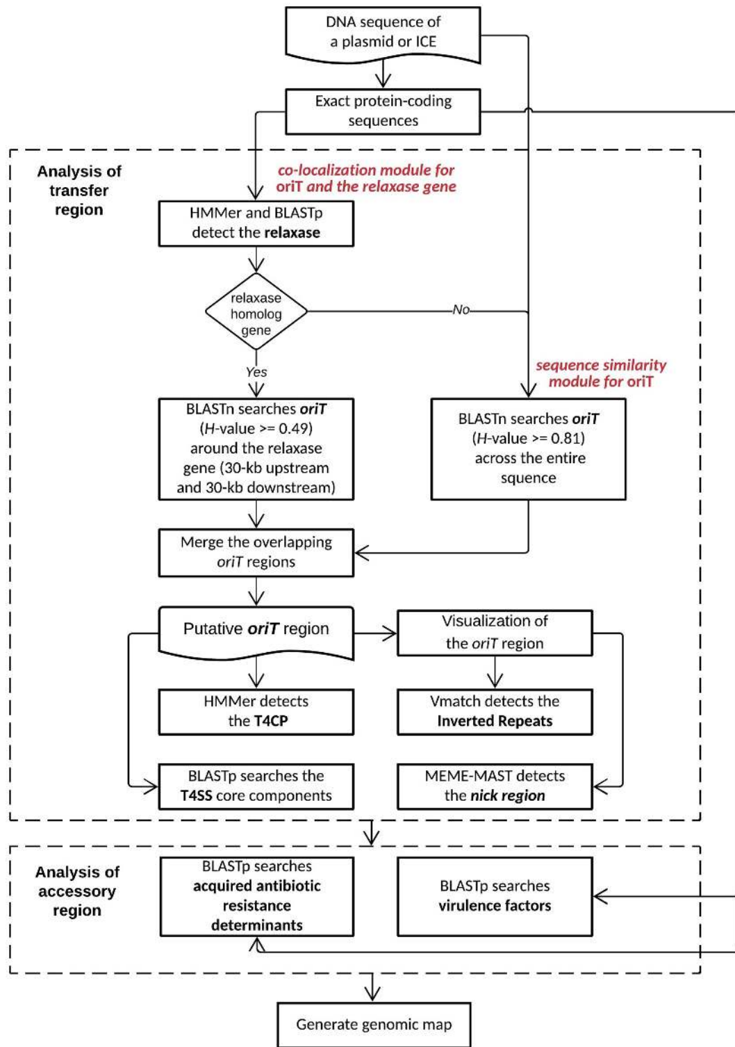
Figure 1. The prediction strategy used by oriTfinder to identify the putative oriT region of a conjugative plasmid or a chromosome-borne ICE. It combines the similarity searches of the oriTDB-archived oriT nucleotide sequence with the co-localization of the flanking relaxase gene.
