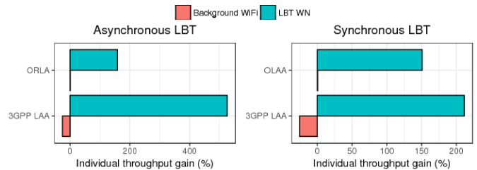
Fig. 7: Individual throughput gain with respect to legacy WiFi in a multi-rate scenarios where an LBT WN share the channel with 5 saturated WiFi WNs. WiFi’s MCS \in \{156, 130, 78, 39, 13\} Mb/s, LBT MCS level = 6. WiFi MPDU = 1500B, LBT Frame size = 1ms. Simulation results.
