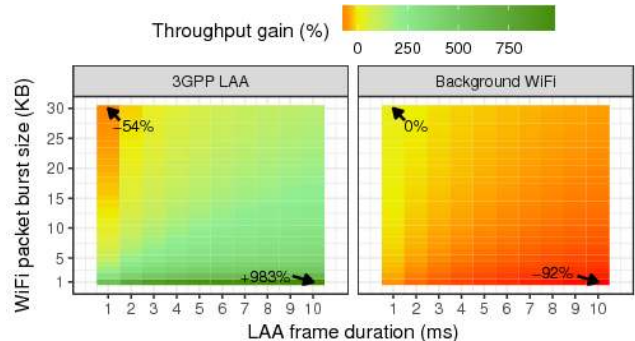
Fig. 1: Throughput gain/loss experienced by a 3GPP LAA transmitter (left) and a WiFi contender (right) in a scenario with one LAA and 5 WiFi transmitters, wrt. a scenario with 6 WiFi transmitters (with packet burst size indicated by the y-axis) and no LAA. Simulation results for different LAA frame sizes (x-axis) and levels of frame aggregation employed by WiFi (y-axis). Both technologies transmit as much data as possible with the same modulation (64-QAM) and contention window configuration. LAA provides gains only if harming WiFi (unfair).
