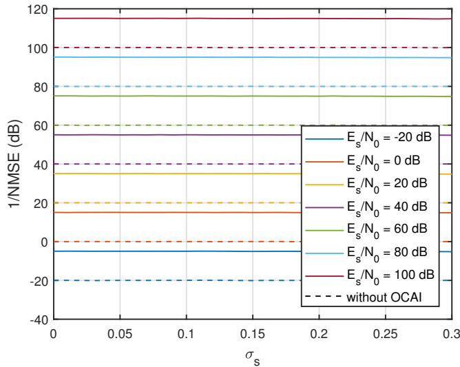
Fig. 4. Comparison of the 1/NMSE performance with and without OCAI as a function of code amplitude imbalance for different E_s/N_0 levels.
