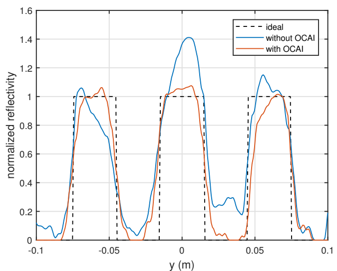
Fig. 11. Measured reflectivity across the three metal strips comprising the 30 mm resolution target (upper half of Fig. 9) with and without OCAI.
