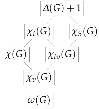
Figure 1: The chromatic numbers and their bounds
