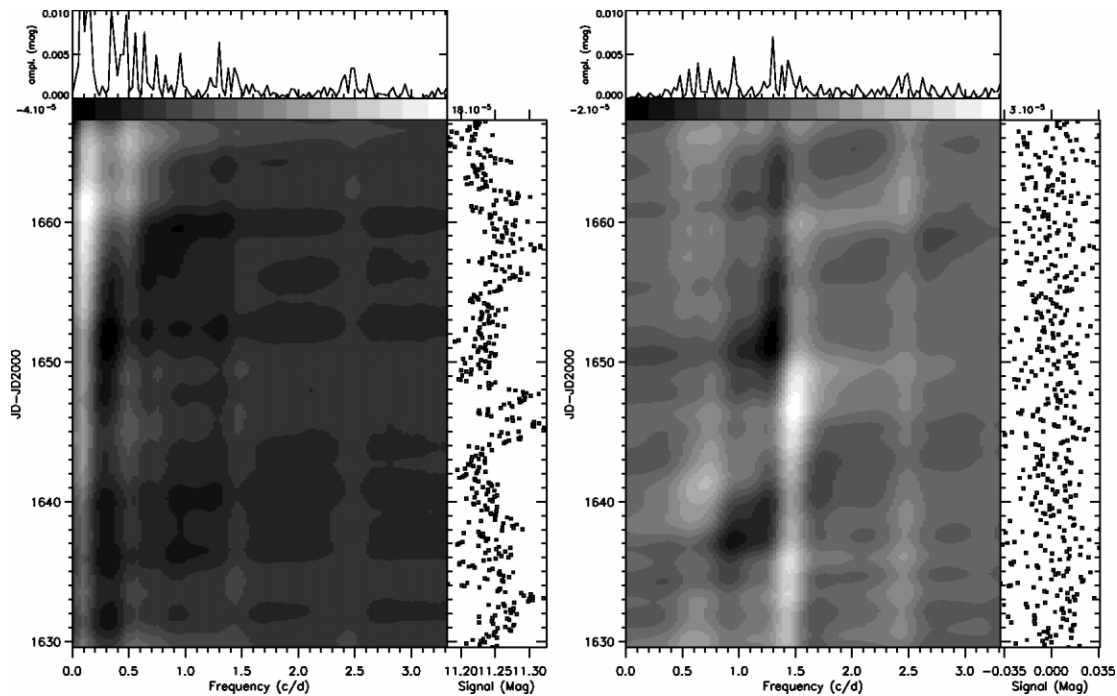
FIG. 2.—Time-frequency analysis of the WR 123 data for the whole set. Left : Data set binned every 2 hr. The upper panel represents the CLEANed spectrum of the whole set and the panel at right is the binned light curve. Right : Data binned every 2 hr and prewhitened, where all signals with P > 1 day have been removed with a high-pass filter. The upper panel is the CLEANed spectrum, and the panel at right is the binned and detrended light curve. The gray-scale calibration is given with lower and upper limits above each gray-scale plot.
