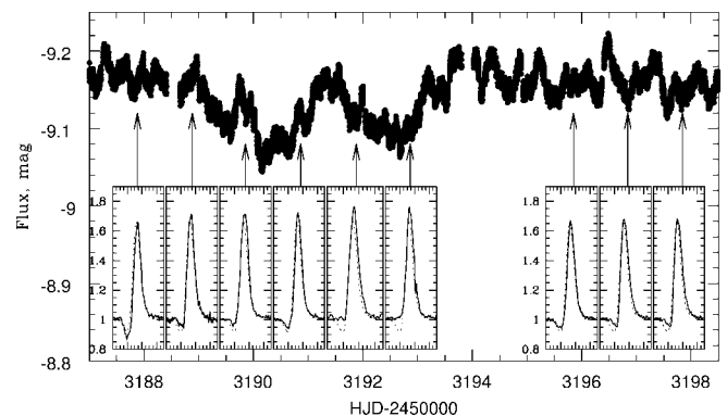
FIG. 3.—Simultaneous spectroscopy from CTIO: the He II 5412 \text{ \AA} line. Dotted lines show an average line profile of the spectra obtained 1 yr before the MOST run.
