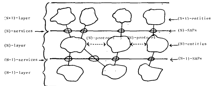
Fig. 4. Entities, service access points (SAP's), and protocols.
