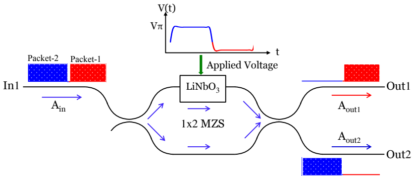
Figure 6.1: Working principle of a 1 \times 2 \text{LiNbO}_3 based electro-optic switch.
