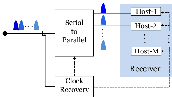
Figure 3.8: Basic OTDM receiver: high-capacity data aggregated from N tributary channels is converted back to M lower base rate tributaries using an optical demultiplexer and detected by M receivers. A clock recovery circuit extracts the base rate control that can be used to synchronize the demultiplexer and receiver.
