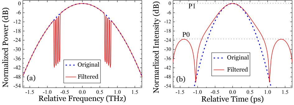
Figure 4.4: (a) Normalized power spectra of a chirp-free 33% RZ-Gaussian optical pulse before (dashed line) and after (solid line) eight optical ONFs (see Figure 4.2(b)) are applied. (b) Normalized intensity profiles of the Gaussian pulse before (dashed line) and after (solid line) notch-filtering.
