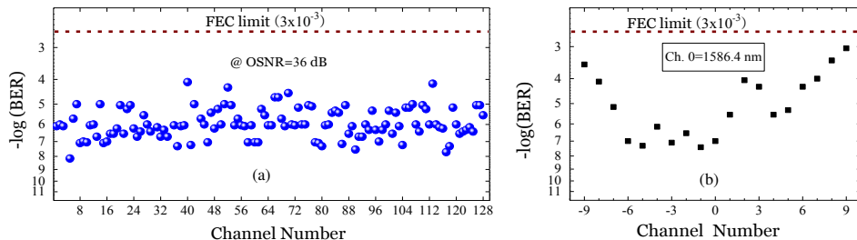
Figure 3.15: (a) BER measurements of all the 128 tributary channels of the 1.28 Tbit/s data packet. (b) BER measurements of simultaneously demultiplexed 19 tributary channels.
