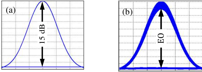
Figure 4.5: Eye diagrams of a 640 Gbit/s RZ-OOK serial data: (a) with EO of 15 dB, and (b) after eight ONFs (refer Figure 4.2(b)) are applied on the data spectrum that leads to EO < 15 dB.
