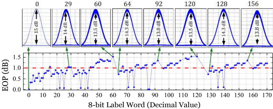
Figure 4.6: The low part shows EOP of the longest packet for LWs up to decimal value of 170, above which the EOP remains > 1.12 dB but below 2.2 dB. The upper part shows eye diagrams of selected LWs with their EO .
