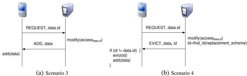
Figure 3. Steps for Update-based Poll-Each-Read access scheme in different scenarios when requested object is not locally cached: (a) Scenario 3 and (b) Scenario 4.
