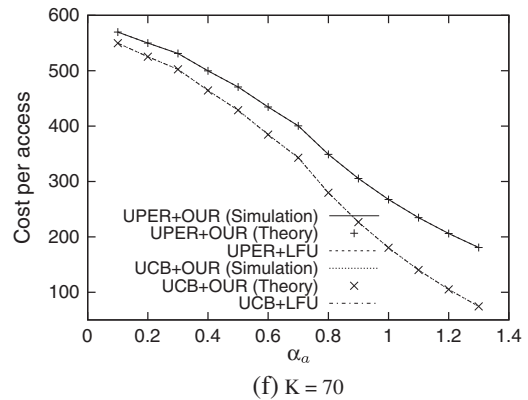
Figure 6. Performance of Optimal Update-based Replacement (OUR) and Least Frequently Used (LFU) for objects with the same update frequencies: (a) K = 50 , (b) K = 60 , (c) K = 70 , (d) K = 50 , (e) K = 60 , and (f) K = 70 . UPER, Update-based Poll-Each-Read; UCB, Update-based Call-Back.
