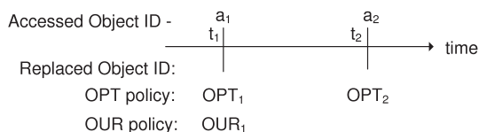
Figure 5. Replacement in Optimal Update-based Replacement (OUR) and other schemes.
