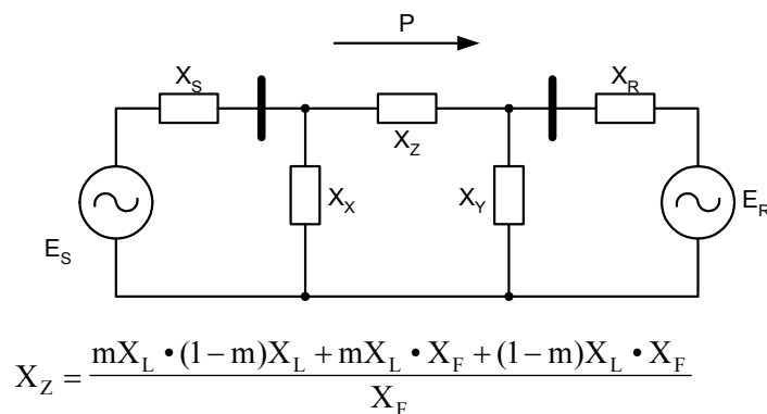
Figure 5 Delta-Wye Equivalent of the Faulted System
