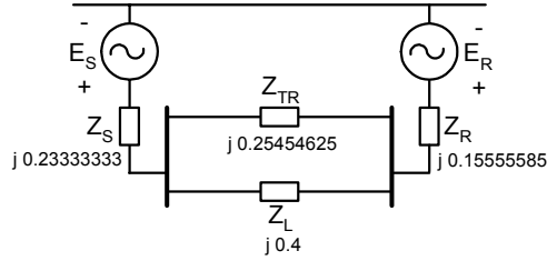
Figure A4 Equivalent Network Between Buses 2 & 3
