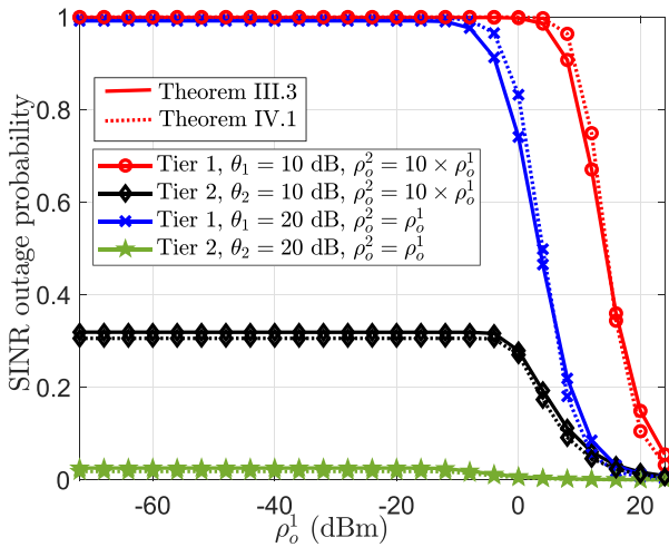
Fig. 7. Dense network approximation of the SINR outage probability in a two-tier mmWave network with \alpha_T^1 = 2 , \alpha_N^1 = 4 , \alpha_T^2 = 2.9 , \alpha_N^2 = 5 , R_B = 200 m, \lambda_0 = 100 , \lambda_2 = 2\lambda_1 , G_{b1}^{\max} = 10 dB, and G_{b2}^{\max} = 7 dB.
