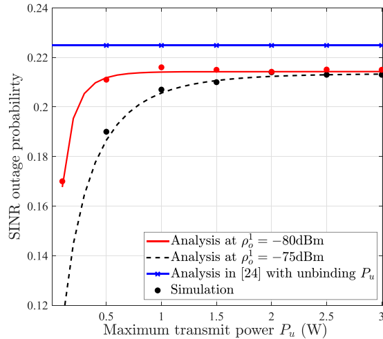
Fig. 3. Effect of the maximum transmit power in a single-tier mmWave network for \theta_1 = 20 dB, \beta_1 = 0.0071 , \alpha_L^1 = 2 , \alpha_N^1 = 4 , and BS densities \lambda = 10 BS/km 2 .
