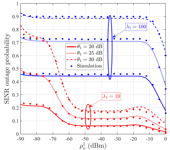
Fig. 4. Effect of the BS density on the SINR outage probability for \lambda_1 = 10 and 100 BS/km 2 , \beta_1 = 0.0071 , \alpha_L^1 = 2 , and \alpha_N^1 = 4 in a single-tier network.
