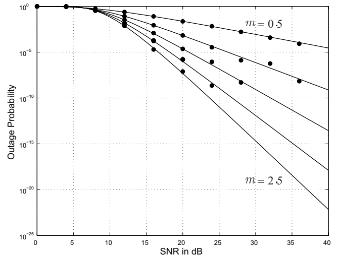
Fig. 2. Outage probability against the transmitted SNR for m = 0.5, 1, 1.5, 2 , and 2.5 . Simulations are shown with dots. In all cases a = 2 .
