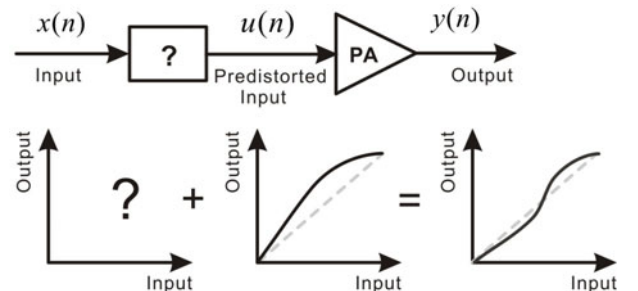
Fig. 5. The new scenario for the output-controllable DPD.
