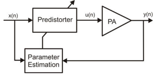
Fig. 4. Direct learning architecture.
