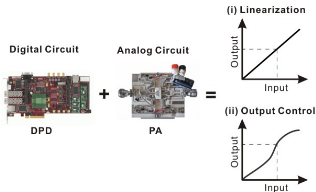
Fig. 1. Digitally assisted analog design example: digital predistortion of power amplifier (i) Conventional linearization (ii) New output-controllable DPD.
