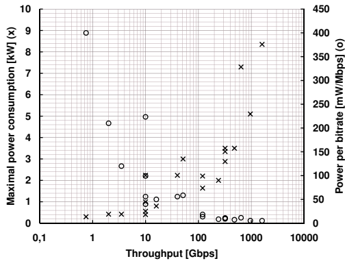
Figure 2. Maximal Power consumption ( \times ) and power per bitrate ( \circ ) of routers versus the maximal throughput
