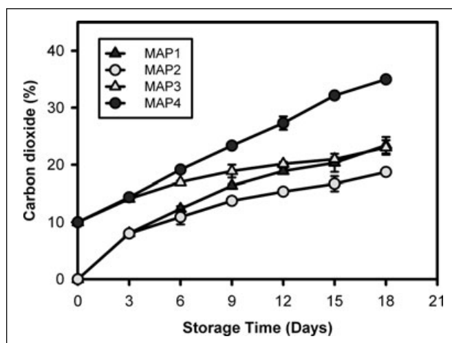
Figure 2—Effect of modified atmosphere packaging (MAP) on the headspace carbon dioxide concentration (%) during storage. (MAP1: 21% O 2 , 79% N 2 ; MAP2: 100% N 2 ; MAP3: 5% O 2 , 10% CO 2 , 85% N 2 ; MAP4: 70% O 2 , 10% CO 2 , 20% N 2 . Points without error bars are smaller than symbols.)
