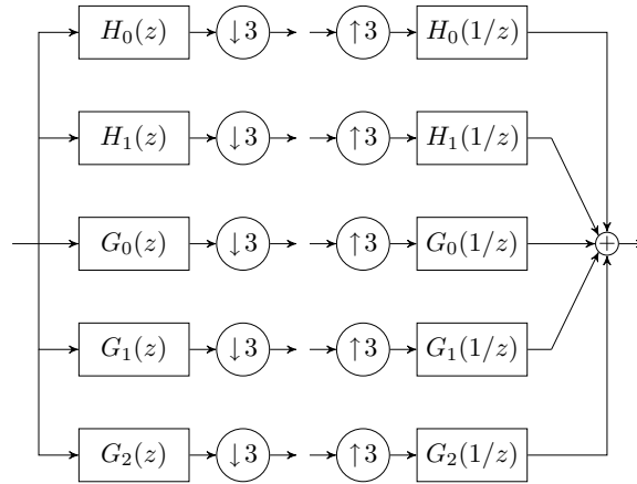
Fig. 9. A filter bank that is equivalent to the one in Fig. 8.
