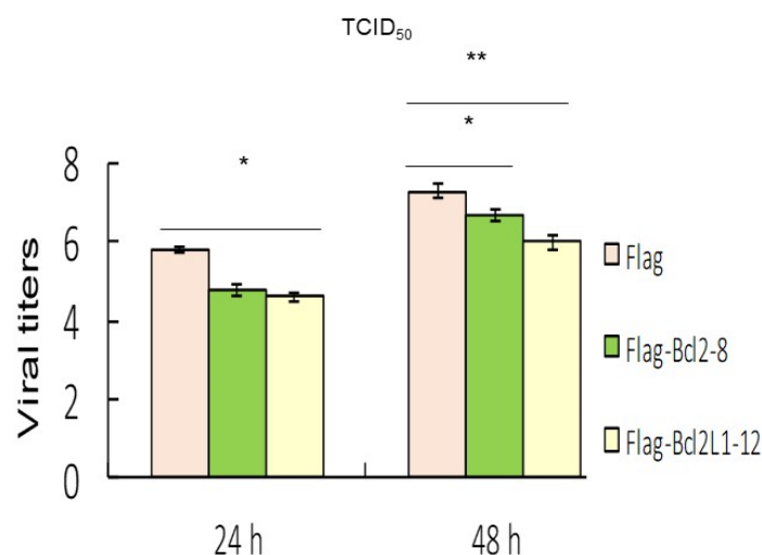
Figure 5. Overexpression of Bcl2 and Bcl2L1 suppressed viral replication. Viral titers (determined by the TCID 50 assay) in the supernatants of different groups at 24 and 48 h, which received best effect on reducing titer between 50 to 100 times by Bcl2 or Bcl2L1 overexpression in three separate experiments. * p < 0.05 ; ** p < 0.01 .
