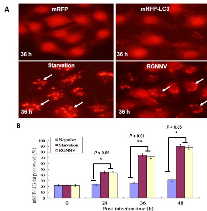
Figure 1. RGNNV-induced autophagosome formation in GF-1 cells. (A) The formation of autophagosomes in GF-1 cells at 36 h detected by the mRFP-LC3 reporter system, with which the formation of RFP-LC3 puncta or dots was counted up to 10 as a positive cell.; mRFP (negative control), mRFP-LC3, serum-starvation treatment, and RGNNV infection. Arrows indicated autosomes. Scale: 10 \mu M. (B) Quantification of the results in A at 0 h, 24 h, 36 h and 48 h in three separate experiments, based on 200 cells per treatment. Results are shown as means \pm SEMs. * p < 0.05 , ** p < 0.01 .
