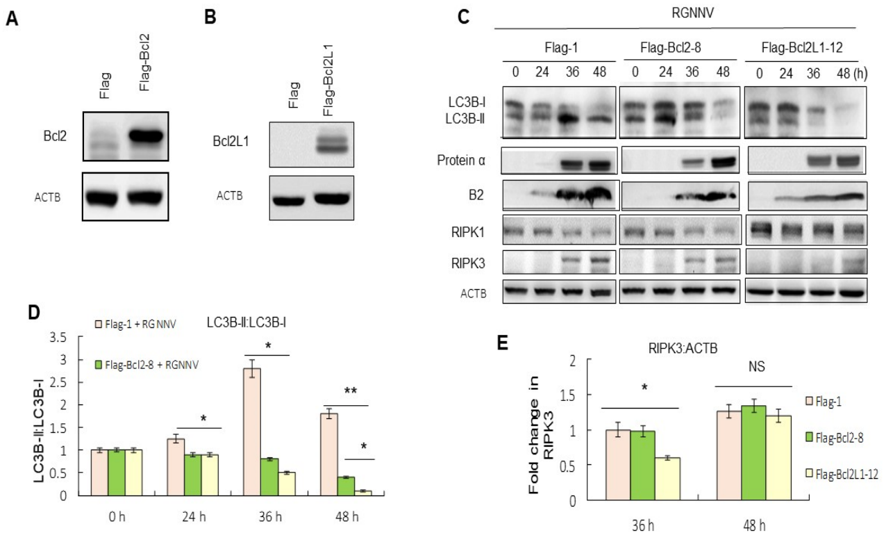
Figure 3. Overexpression of Bcl2 and Bcl2L1 suppressed autophagy and necroptosis. (A,B) Western blot analysis of Bcl2- and Bcl2L1-producing cells was identified by Bcl2 and Bcl2L1 PolyAbs. (A) Lanes: 1, Flag alone; 2, Bcl2-producing cells. (B) Lanes: 1, Flag alone; 2, Bcl2L1-producing cells. (C) Western blot analysis showed the effect of Bcl2 and Bcl2L1 overexpression on autophagy, necroptosis and viral replication, based on the LC3-II:LC3-I ratio, RIPK3 expression and viral protein expression. Lanes: 1–4, RGNNV-infected Flag-producing GF-1 cells at 0, 24, 36, and 48 h; 5–8, RGNNV-infected Bcl2-producing GF-1 cells at 0, 24, 36, and 48 h; 9–12, RGNNV-infected Bcl2L1-producing GF-1 cells at 0, 24, 36, and 48 h. (D) Quantitation of the results in C for LC3-II:LC3-I ratio. (E) Quantitation of the results from C showed the effect of Bcl2 and Bcl2L1 overexpression on necroptosis, based on RIPK3 expression at 0, 24, 36, and 48 h in three separate experiments. Results are shown as means \pm SEMs. * p < 0.05 ; ** p < 0.01 .
