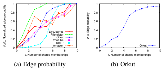
Figure 2: (a) Normalized edge probability as a function of common memberships k . Probabilities are scaled so that maximum value over k is one. (b) Edge probability in the Orkut network, plotted as an absolute value. We conclude overlaps are more densely connected than single communities.
