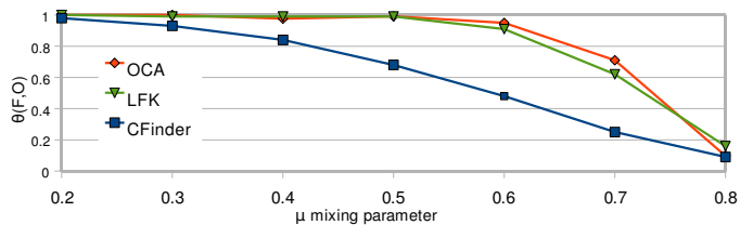
Fig. 2. Evolution of \Theta against \mu .
