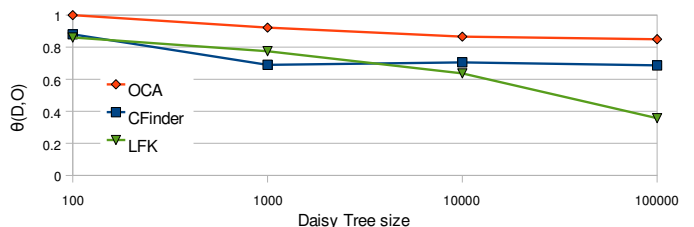
Fig. 3. \Theta of daisy community structure with different sizes
