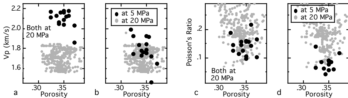
Figure 2. Compressional-wave velocity (a and b) and Poisson's ratio (c and d) versus porosity for North Sea sandstones (black circles) and Gulf sandstones with gas (gray symbols). The North Sea laboratory data are from Blangy (1992); the Gulf sandstone data are from a well log (discussed in Dvorkin et al., 1999) at about 20 MPa differential pressure. In a and c, North Sea data shown at 20 MPa (same as the Gulf data). In b and d, North Sea data shown at 5 MPa (the Gulf data are at 20 MPa).
