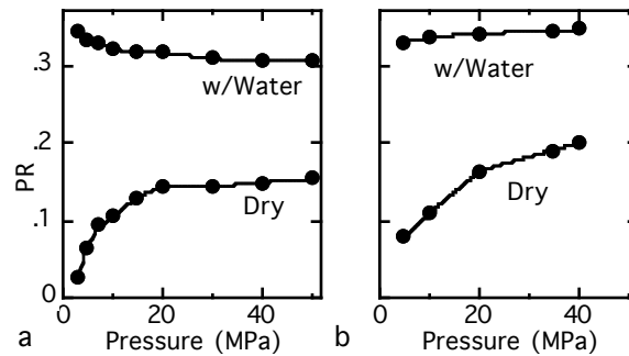
Figure 7. PR in dry and water-saturated samples versus differential pressure for (a) sample used in Figure 3k and (b) sample used in Figure 3h.
