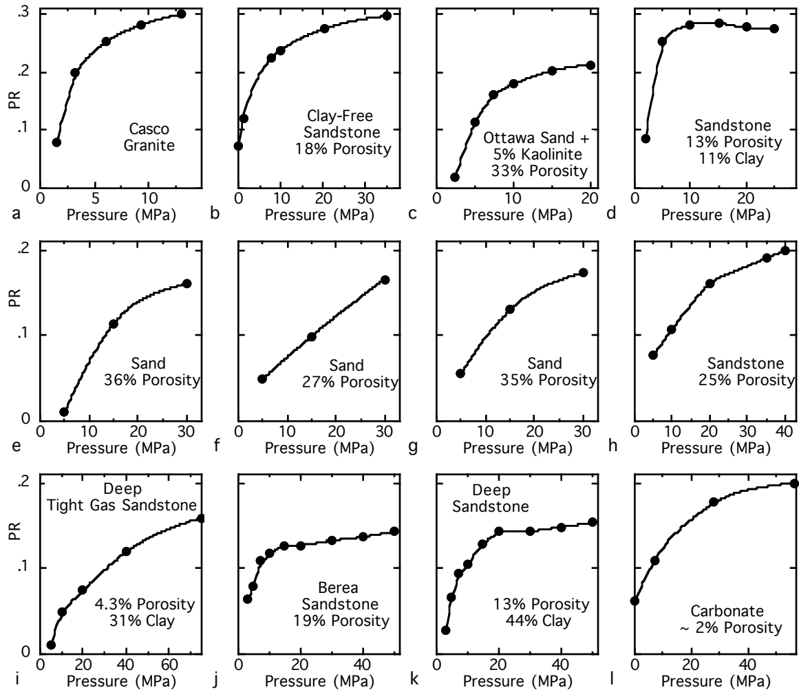
Figure 3. PR versus differential pressure in room-dry samples. Data used are from Nur (1969), Yin (1993), Han (1986), Blangy (1992), and authors' database.
