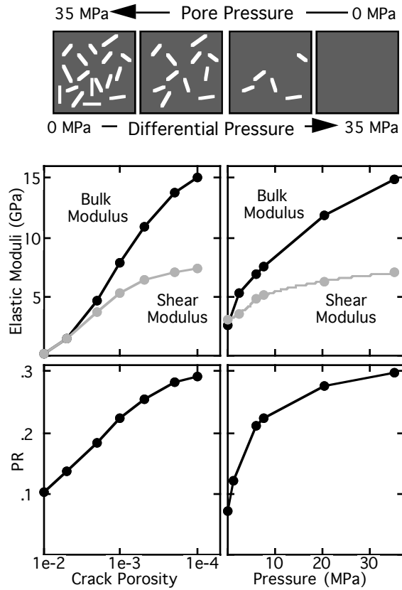
Figure 5. Theoretical modeling of pressure effect on the elastic moduli of the room-dry sandstone sample from Figure 1. Top cartoon: crack opening and closure as pressure changes. Left column: theoretical bulk and shear moduli (top) and PR (bottom) versus crack porosity. Right column: experimental bulk and shear moduli and PR versus differential pressure.
