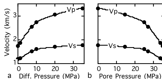
Figure 1. a. Velocity versus differential pressure in ultrasonic laboratory experiments on room-dry clay-free sandstone sample of 18% porosity. b. Same data re-plotted versus (fictitious) pore pressure assuming that the overburden is 35 MPa and differential pressure changes due to changing pore pressure.
