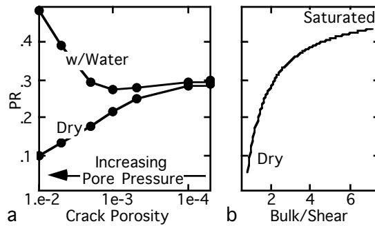
Figure 6. a. Theoretical modeling of pressure effect on the dry-rock and rock-with-water PR in a synthetic calcite sample. PR versus crack porosity. Higher crack porosity corresponds to low differential or high pore pressure. b. PR versus the bulk to shear modulus ratio. The low bulk to shear ratio is typical for dry rock whereas the high ratio is typical for soft fluid-saturated rock.
