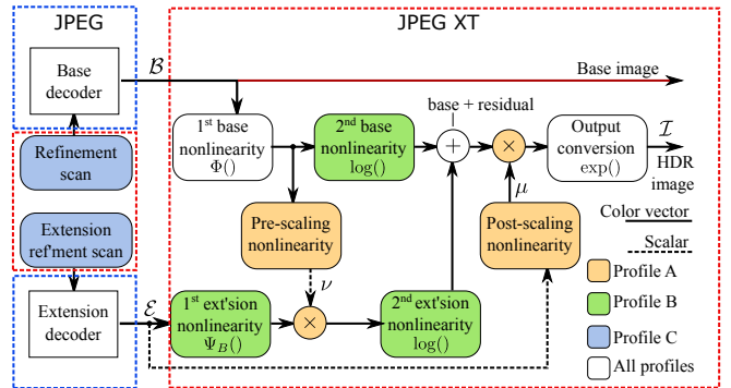
Fig. 2 The simplified JPEG XT standard decoder architecture: (blue-dashed line) is the legacy coding system ISO/IEC 10918/T.81 known as JPEG format - (red-dashed line) are the additional components that define the new JPEG XT standard.
