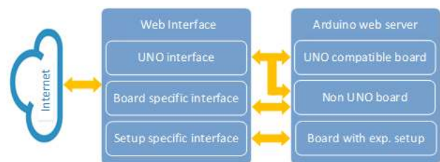
Figure 13. Web interface structure
