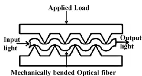
Figure 14. Micro bend sensor concept [40].
