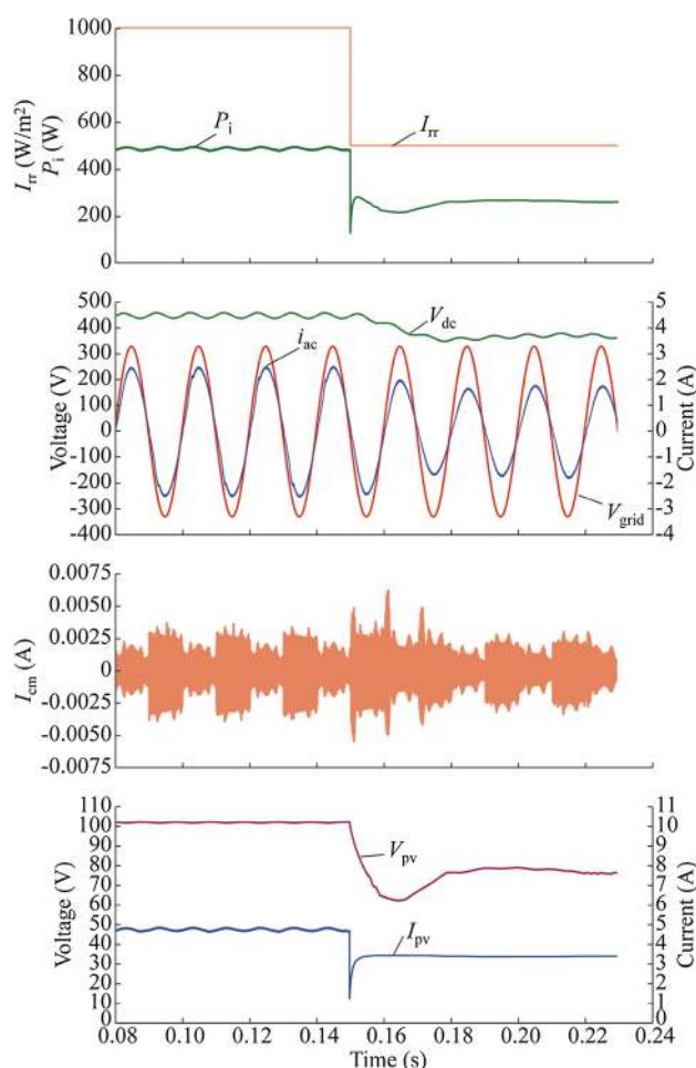
Fig. 11 Performance of proposed PV system by changing irradiance
