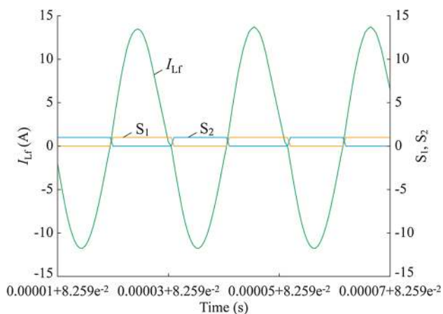
Fig. 8 Current waveform of inductor
