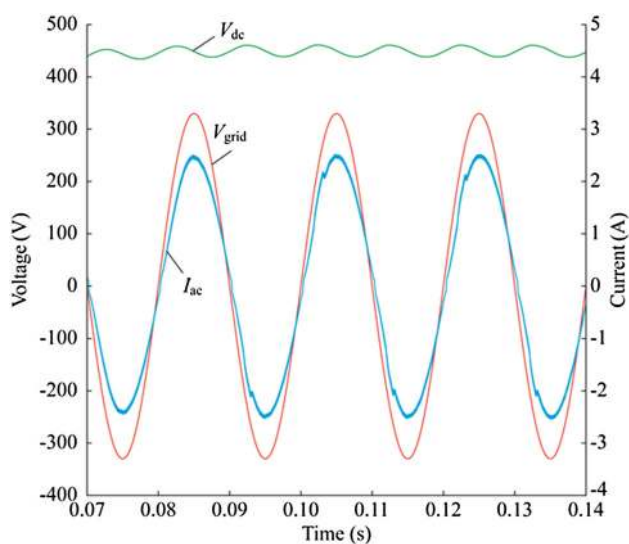
Fig. 9 DC bus voltage and AC currents/voltages waveform
