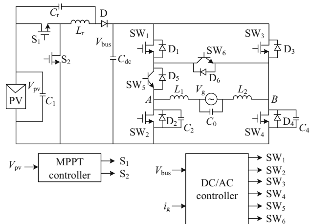
Fig. 6 Proposed two stage PV system
