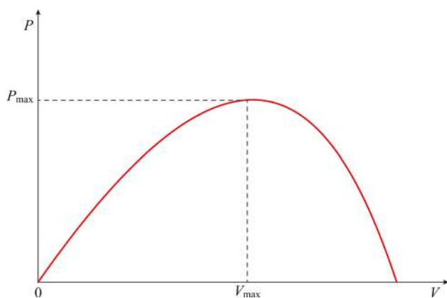
Fig. 5 Characteristic of PV panel power curve
